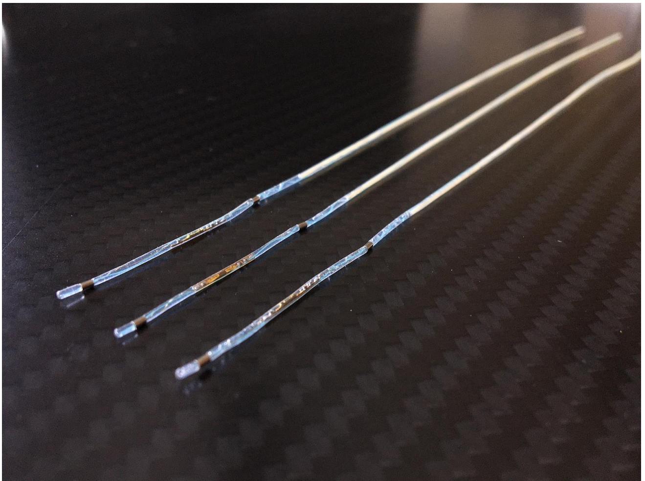
The miniaturized muscle implant, consisting of electrode contacts and electronics, is just three centimeters long and barely one millimeter thick. A silicone tube is used to extract the implant after the experiment.
